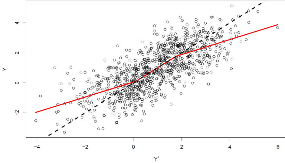
Figure 1.1: Realizations of Y^*, Y when a = b = 0.5 based on a random draw of size n = 1000 . The red solid line depicts the function h and the black dashed line the 45^\circ line.
